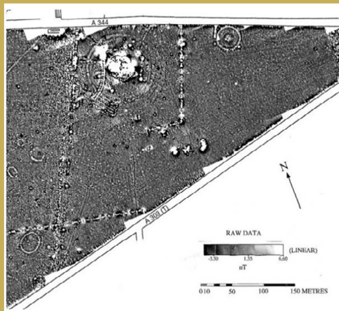
Figure: Thermal survey in Visoko Pyramids, Bosnia (Smailbegovic, 2006)
