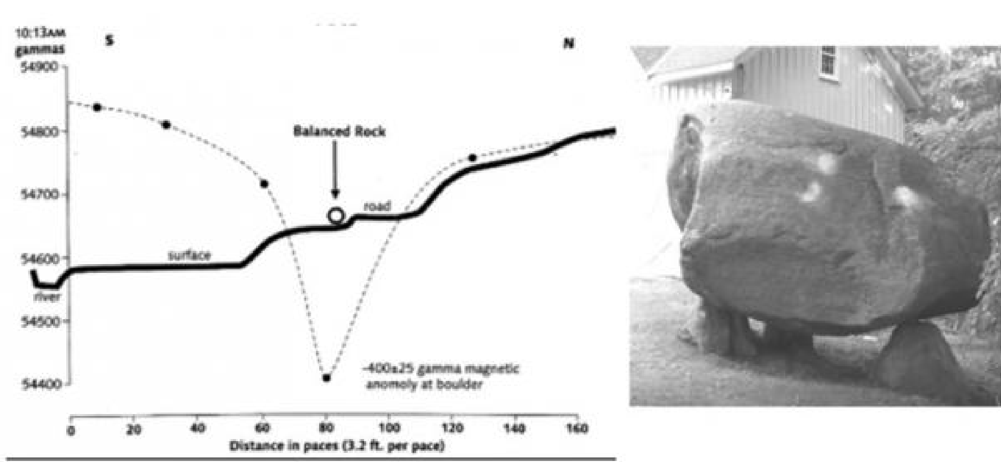
Figure: Geomagnetic field intensity on the location of Balanced Rock (Burke,2005)
